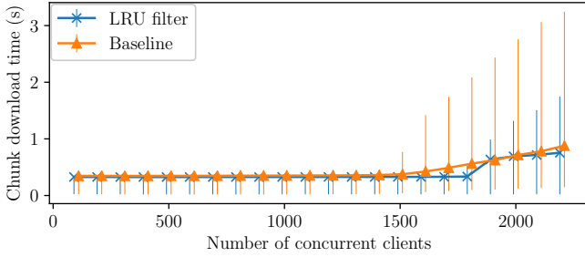
Fig. 12. Median chunk download time versus number of concurrent clients, for N = 10^7 , \alpha = 0.9 , \delta_2 = 0.01 . Error bars represent the 10th and 90th percentiles. In-network LRU filter with \delta_1 = \delta_1^* = 0.06 vs no filter.
